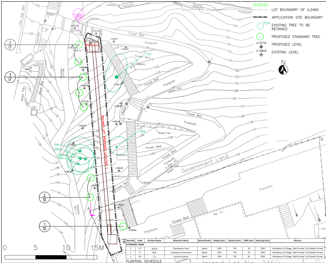
Figure 3.5: Landscape Proposal
