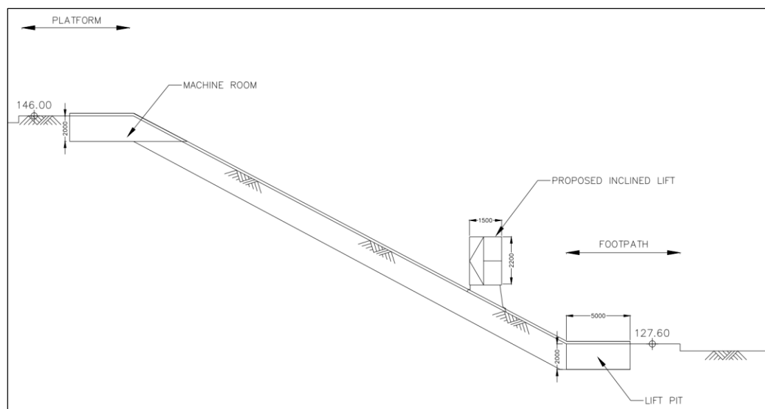
Figure 3.2: Section of The Proposed Inclined Lift
