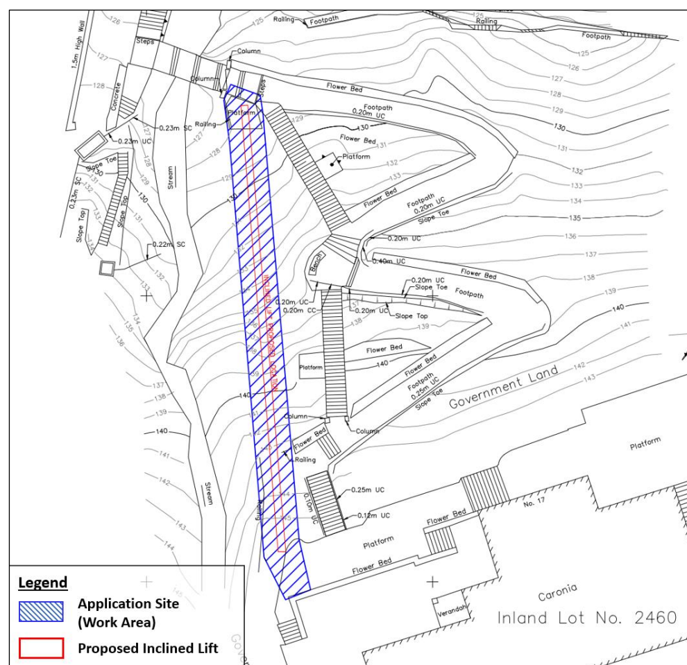
Figure 3.1: The Proposed Inclined Lift
